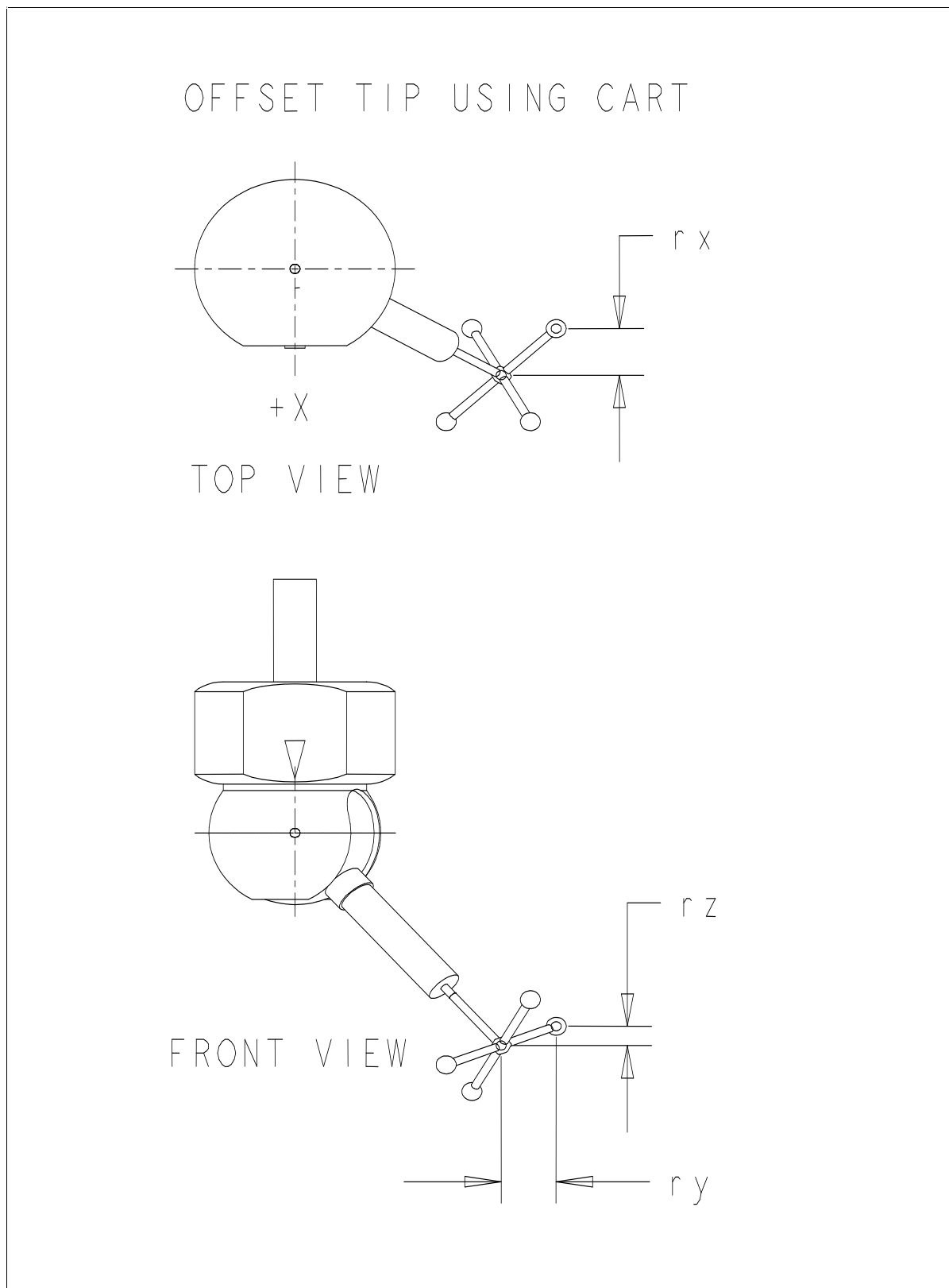
Figure B.75 — Offset tip Cartesian
