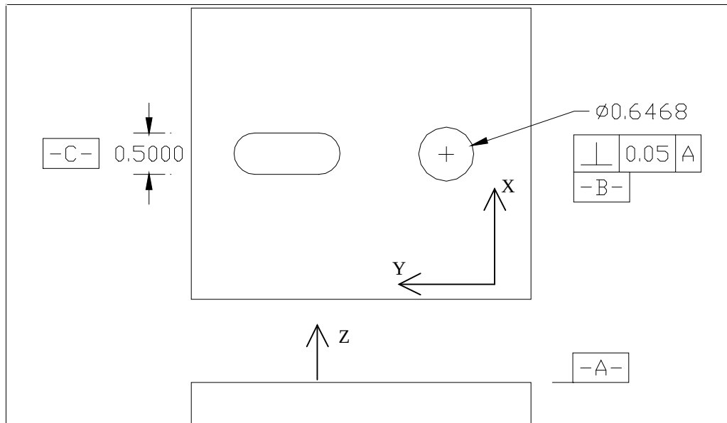
Figure 11 — Plate with a hole and slot
