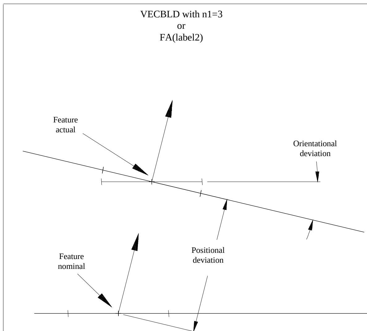
Figure B.47 — Positional and orientational deviation
