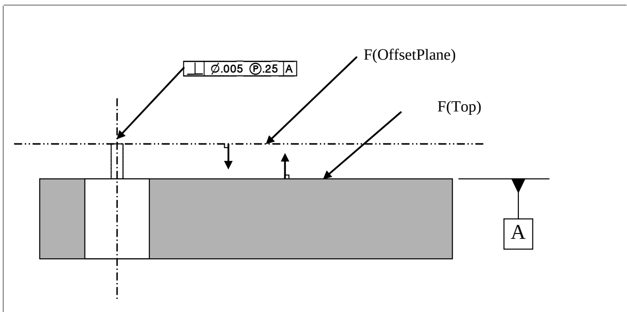
Figure 6 — Tolerance boundaries
