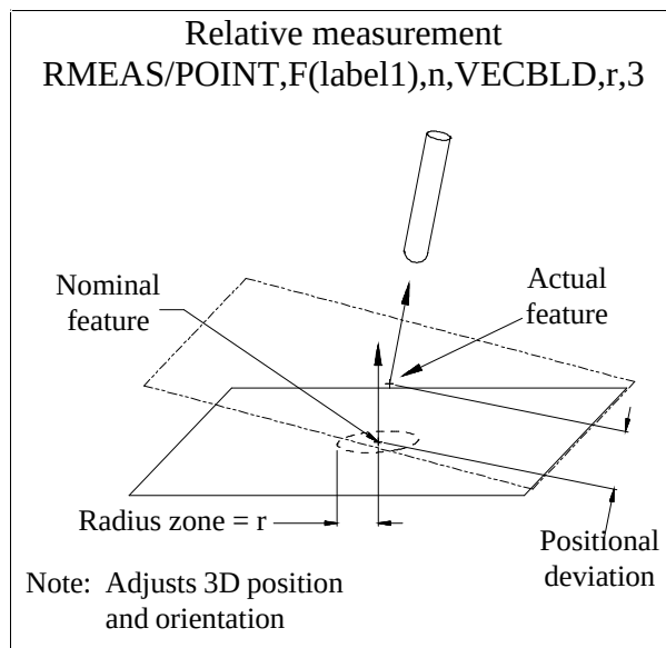
Figure B.65 — RMEAS/POINT with VECBLD,r,3 using a surface point
