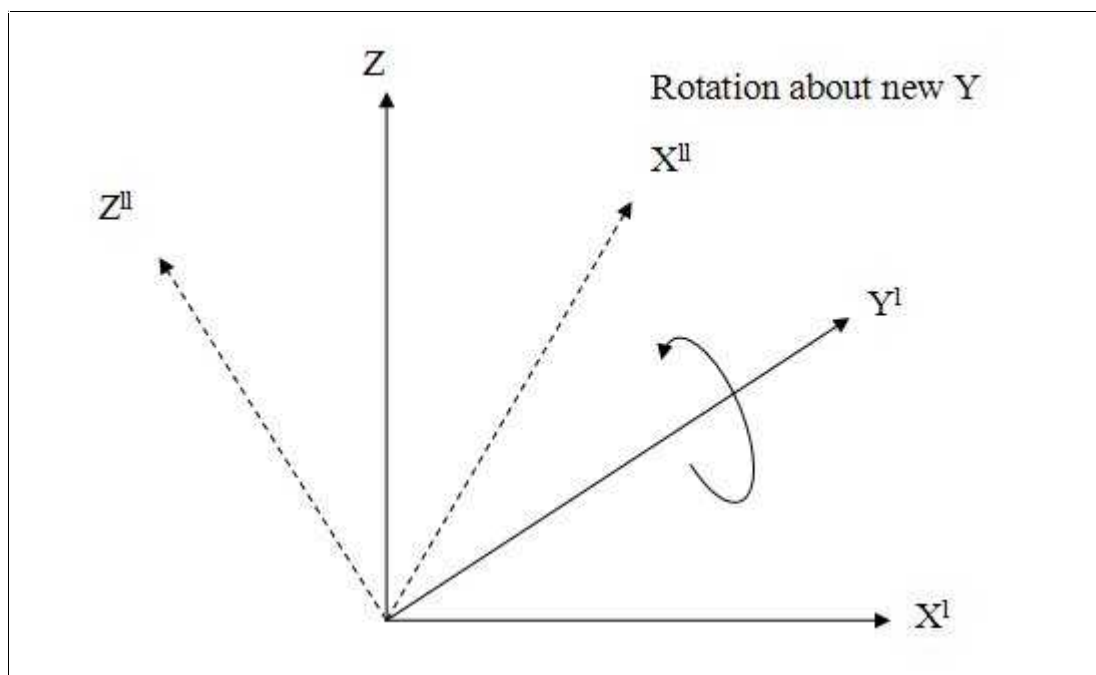
Figure 15 — Euler transformation 2
