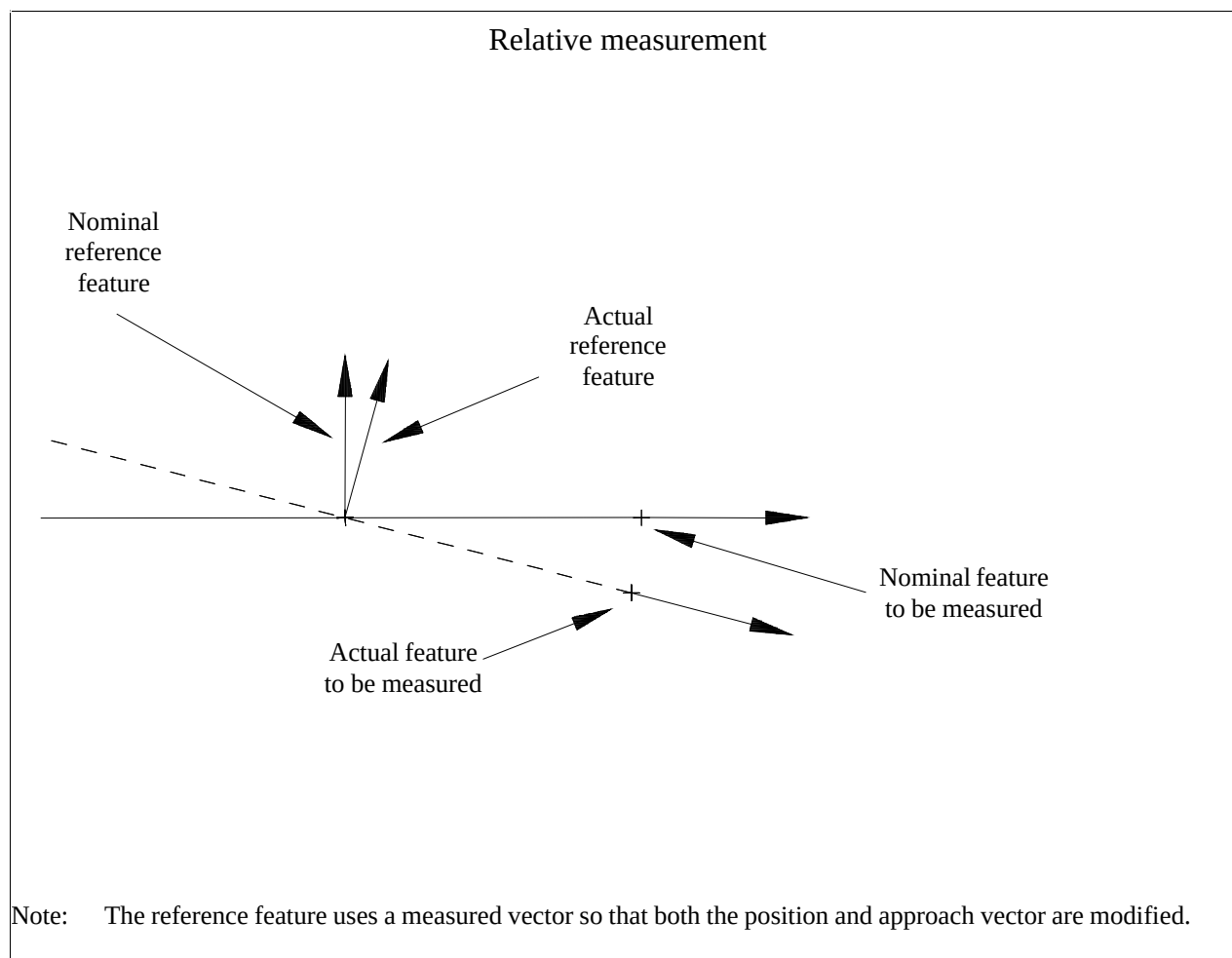
Figure B.48 — Relative measure / position & approach
