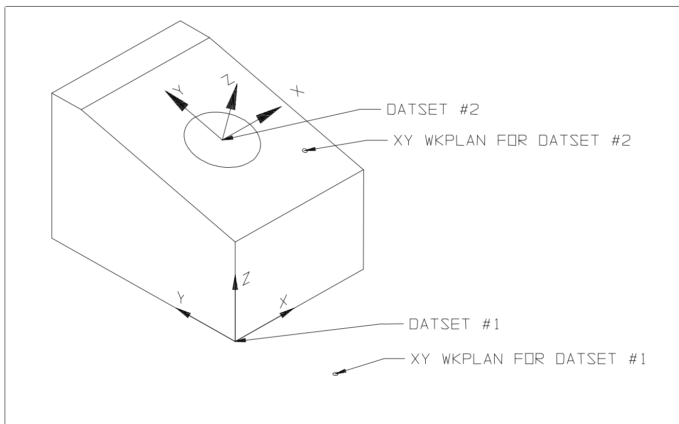
Figure B.89 — Work Plane change as a result of a new DATSET statement execution
