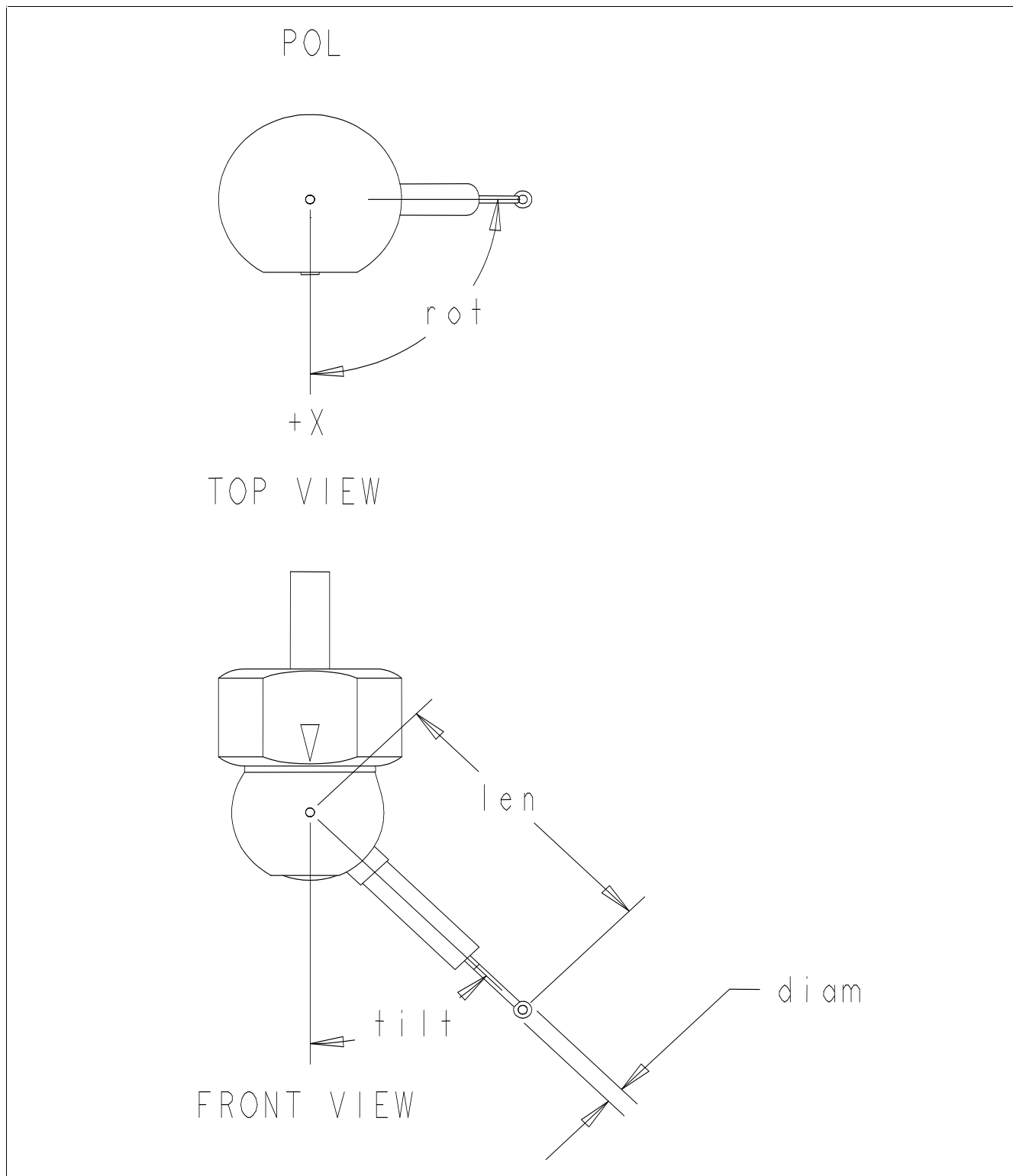
Figure B.73 — Indexable head polar coordinates
