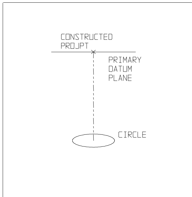
Figure B.13 — Constructed projected point
