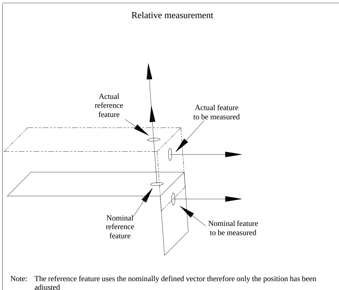
Figure B.50 — Relative measure / position
