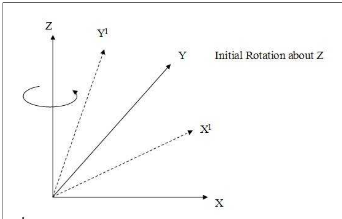
Figure 14 — Euler transformation 1
